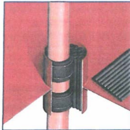
To prevent the filler sleeves from falling out of the conduit sleeve or frame, they are hooked together to form a compact bundle. They are available in bundles of ten pieces. Filler sleeves are also available non-split.
