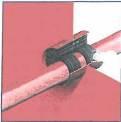
6) The empty space in the conduit pipe should be filled up completely with insert sleeves, types 18/12 and 27/19. The sleeves are 210 mm (8.27") in length and can be supplied non-split for ease of installation.
